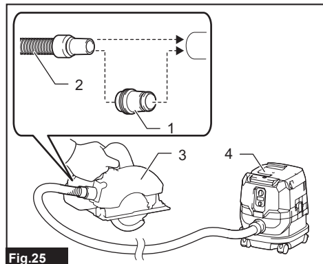
Fig. 25 ► 1. Front cuffs or joint 2. Cleaner hose 3. Power tool 4. Vacuum cleaner
